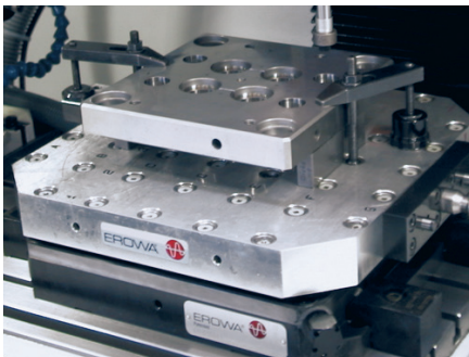
Workpiece holding by EROWA
